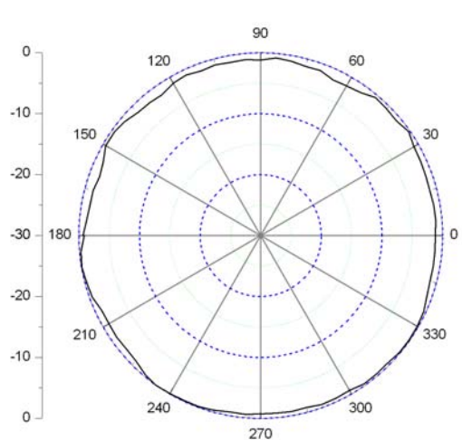
H Plane
