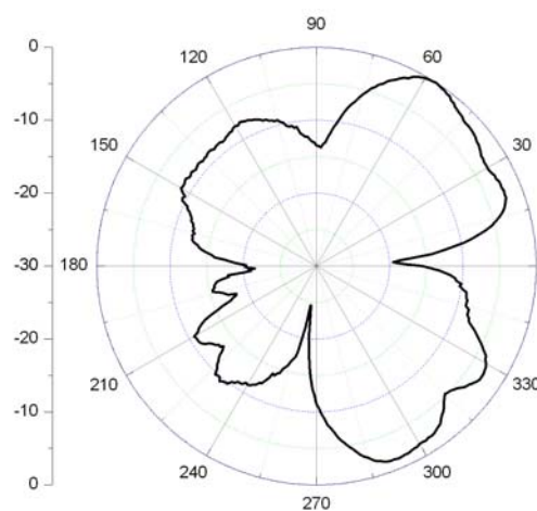
E Plane
