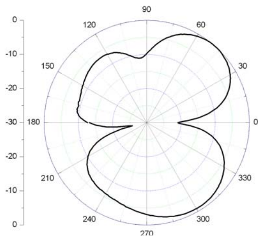
E Plane
