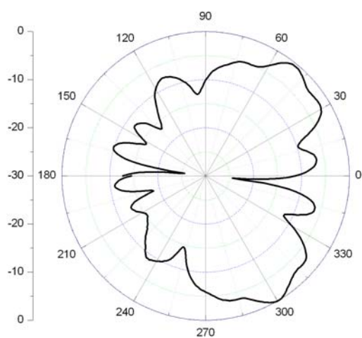
E Plane
