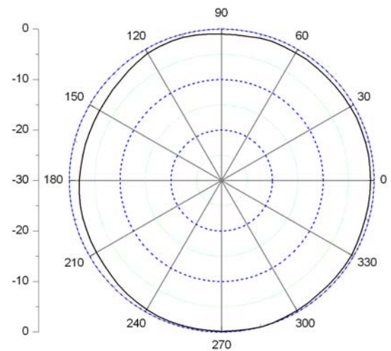
H Plane
